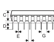
Fig2. 1/2 Lead Packages
