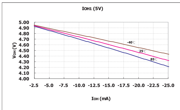
V_{OH} vs. I_{OH1} Over Temperature ( V_{DD}=5.0V )
