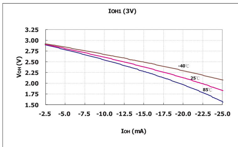
V_{OH} vs. I_{OH1} Over Temperature ( V_{DD}=3.0V )
