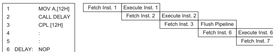
Instruction Fetching
