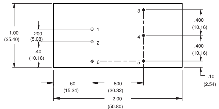
BOTTOM VIEW
