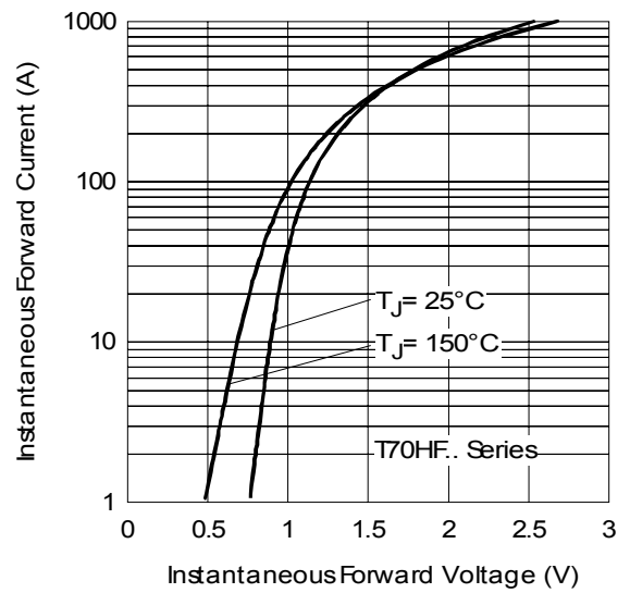
Fig. 26 - Forward Voltage Drop Characteristics
