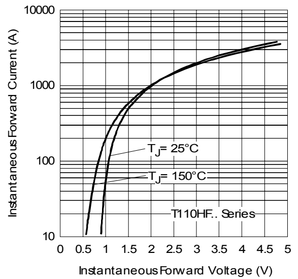
Fig. 28 - Forward Voltage Drop Characteristics
