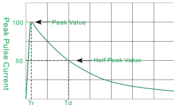
t_r \times t_d Pulse Waveform
