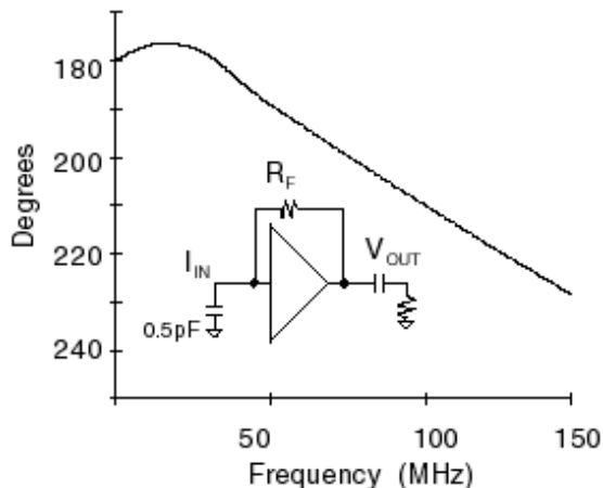
Figure 9: Phase ( I_{IN} to V_{OUT} )
