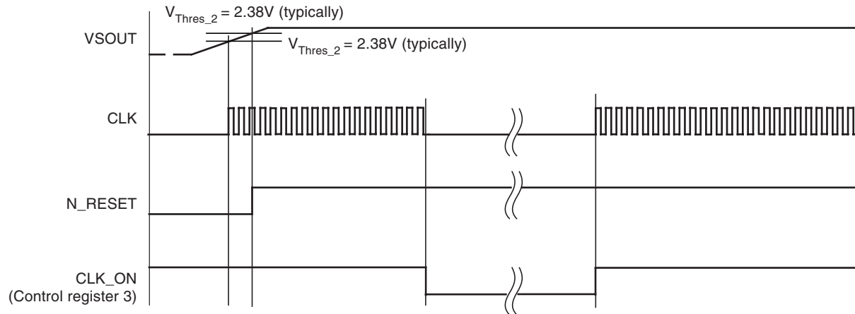
Figure 6-3. Clock Timing
