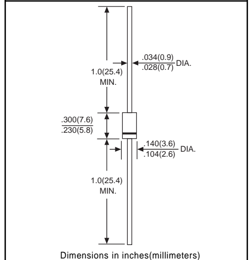
DO-15
