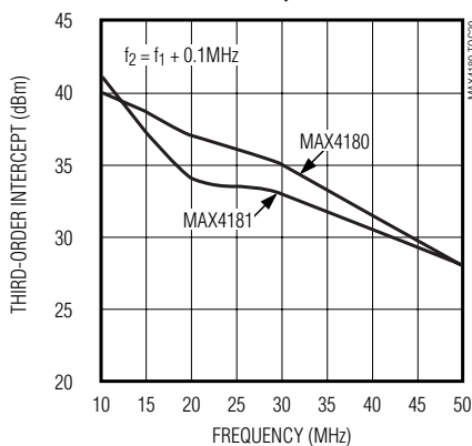
TWO-TONE THIRD-ORDER INTERCEPT vs. FREQUENCY
