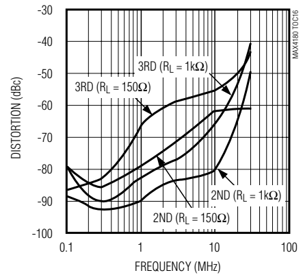
MAX4181 HARMONIC DISTORTION vs. FREQUENCY (SINGLE SUPPLY)
