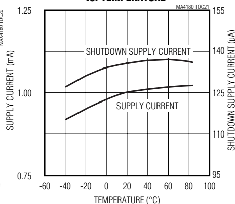
SUPPLY CURRENT (OPERATING & SHUTDOWN) vs. TEMPERATURE
