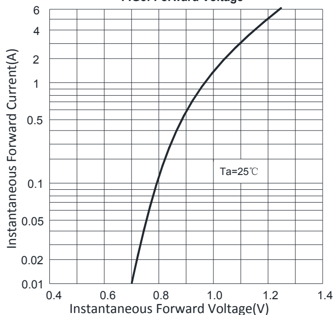
FIG3: Forward Voltage
