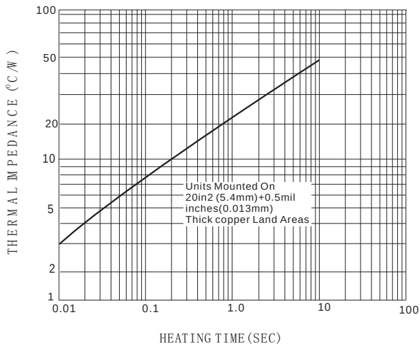
Fig. 5-TRANSIENT THERMAL IMPEDANCE
