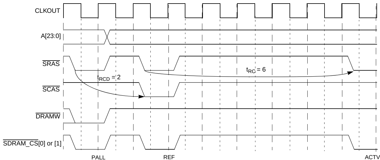
Figure 15-8. Auto-Refresh Operation
