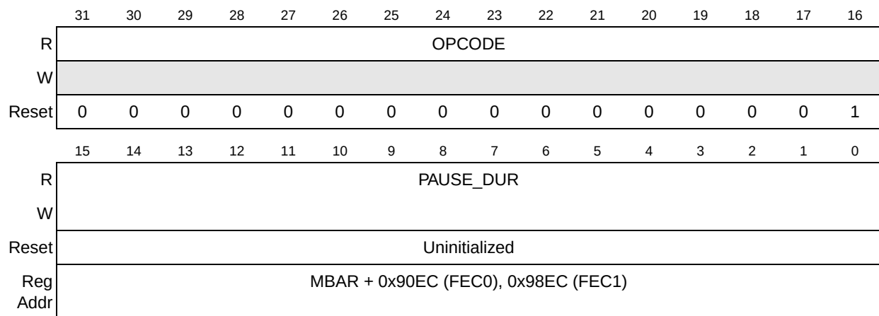
Figure 31-13. Opcode/Pause Duration Register (OPD)
