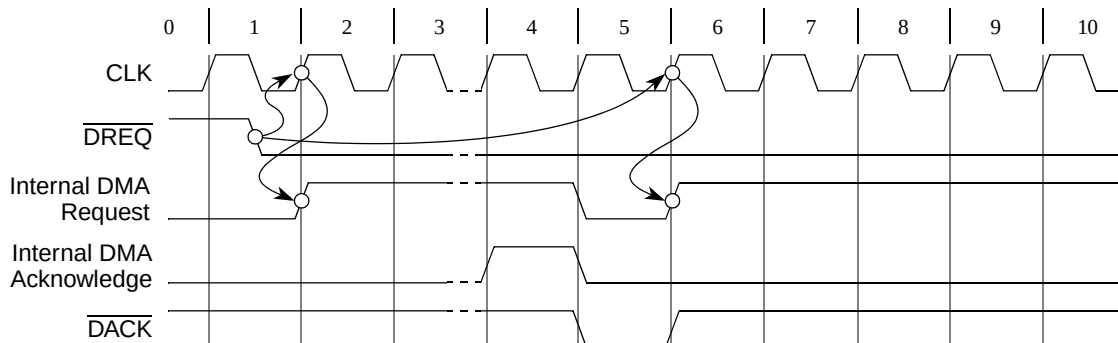
Figure 24-24. Level-Triggered External Request Timing
