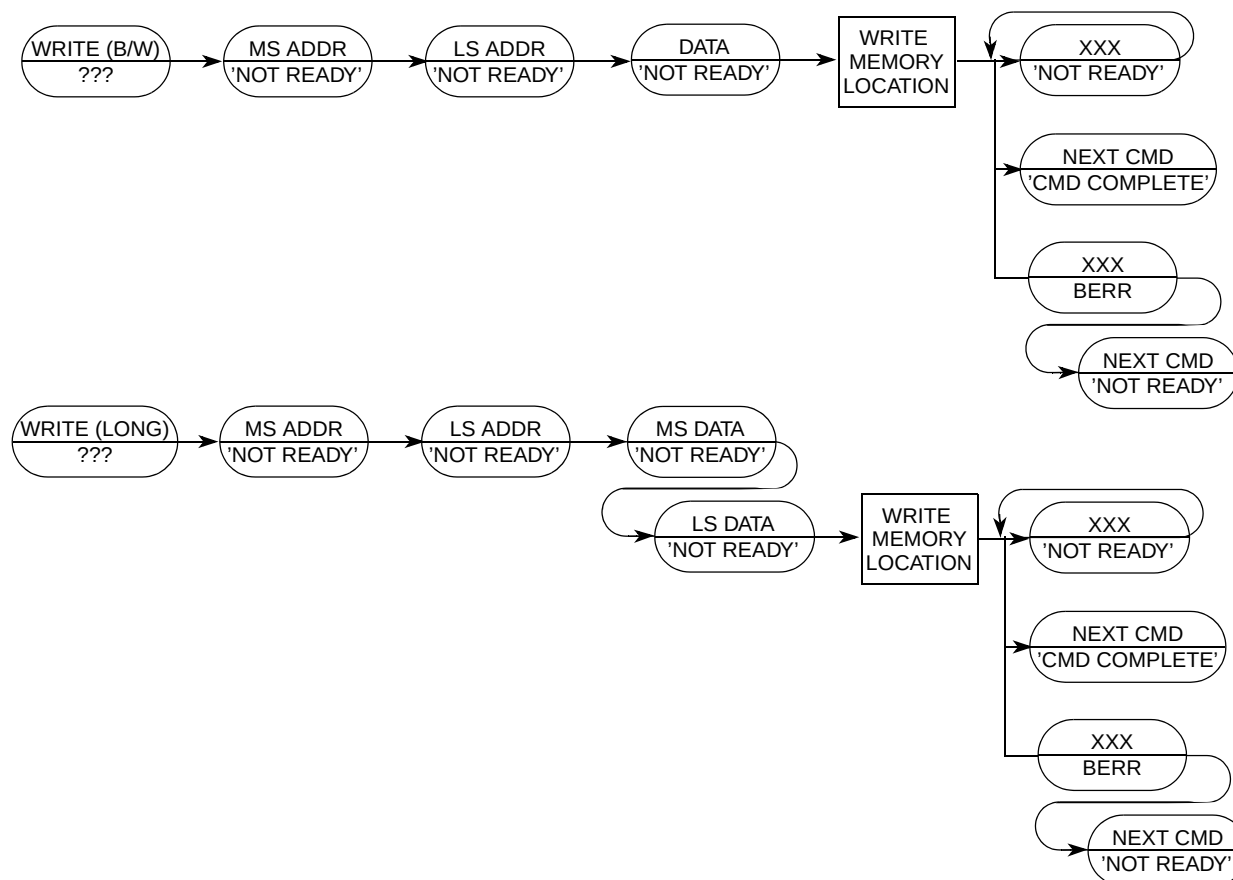
Figure 8-30. WRITE Command Sequence
