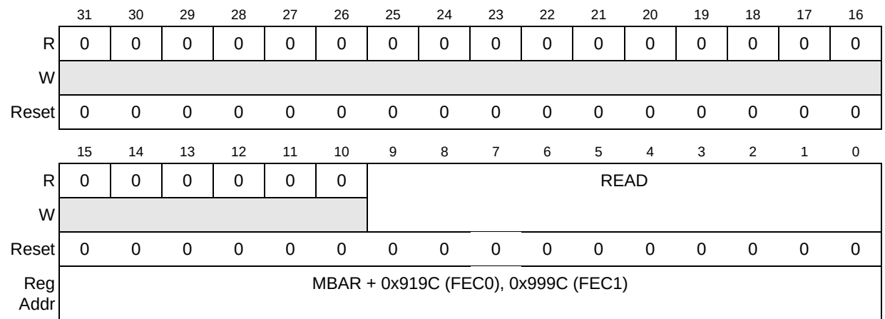
Figure 31-27. FEC Receive FIFO Read Pointer Register (FECRFRP)
