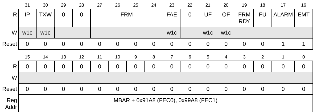
Figure 31-30. FEC Transmit FIFO Status Register (FECTFSR)
