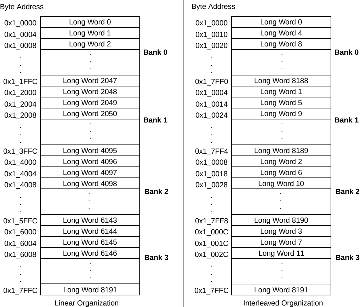
Figure 16-1. SRAM Organization
