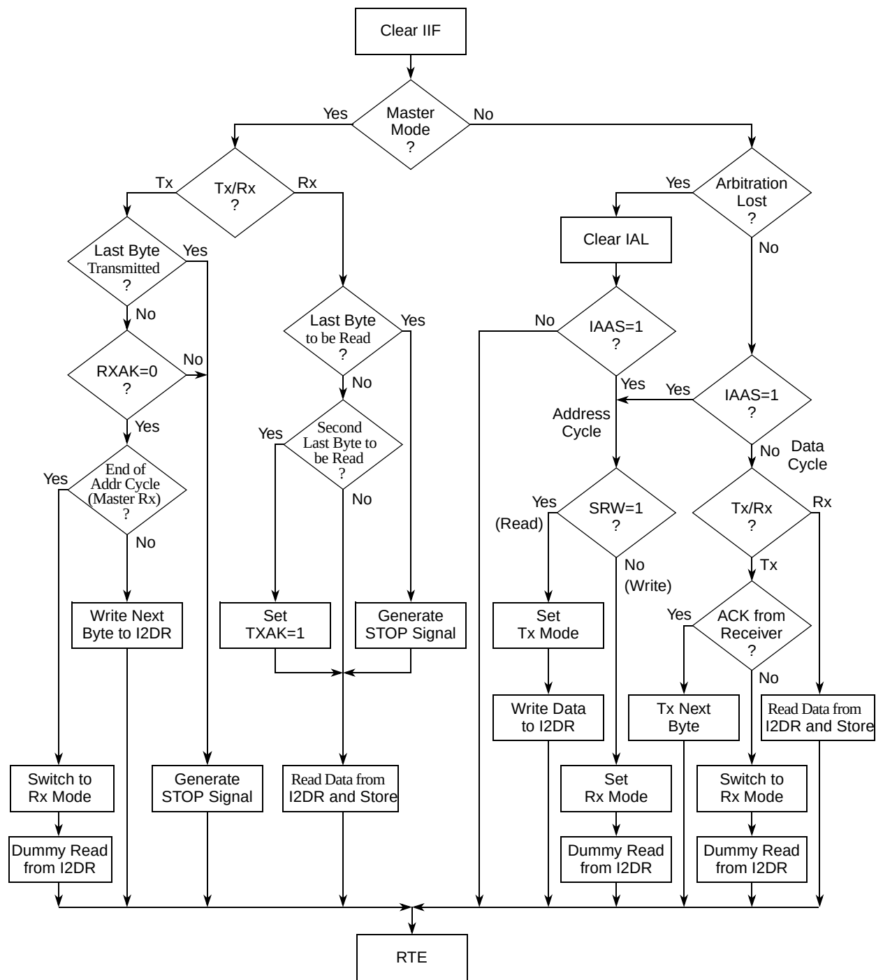
Figure 29-14. Flow-Chart of Typical I²C Interrupt Routine
