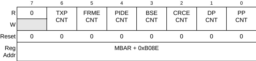
Figure 30-25. USB Counter Overflow Register (CNTOVR)
