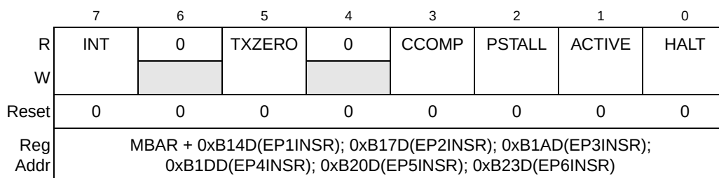
Figure 30-33. Endpoint n Status Register IN (EP n INSR)
