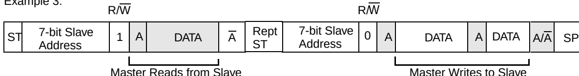
Figure 29-11. Data Transfer, Combined Format
