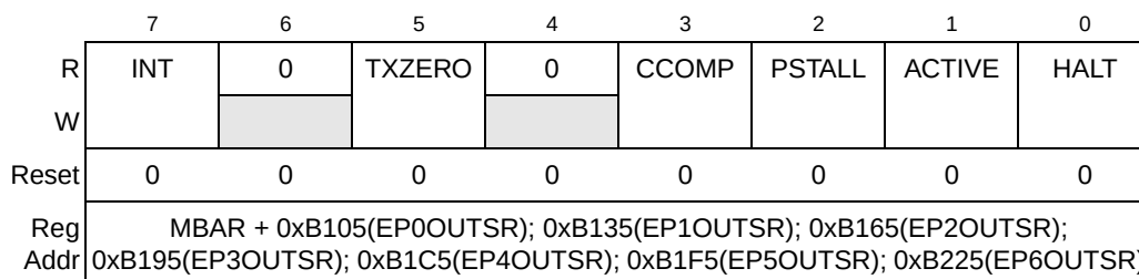
Figure 30-32. Endpoint n Status Register OUT (EP n OUTSR)
