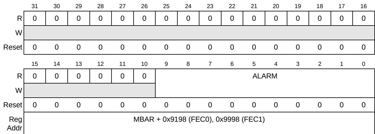
Figure 31-26. FEC Receive FIFO Alarm Register (FECRFAR)
