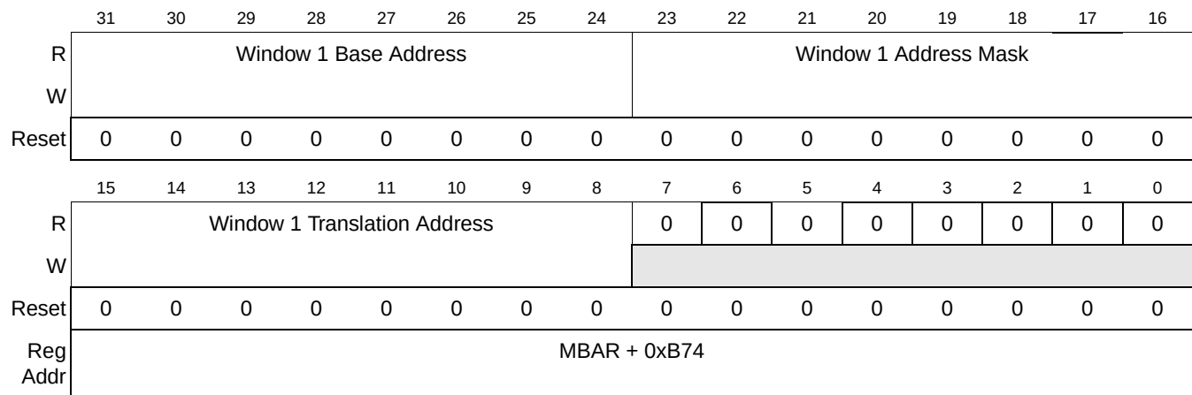
Figure 19-14. Initiator Window 1 Base/Translation Address Register (PCIIW1BTAR)
