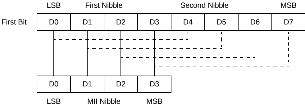
Figure 31-42. MII Nibble/Octet to Octet/Nibble Mapping
