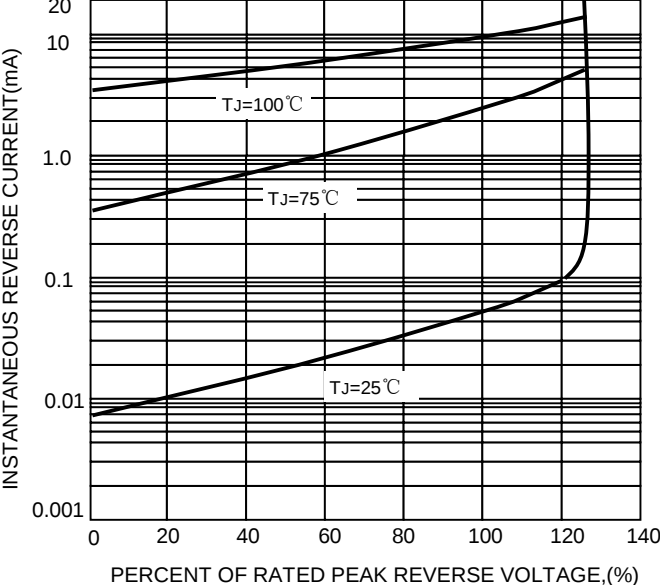
FIG.5-TYPICAL REVER CHARACTERISTICS
