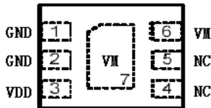
Figure 2. PIN Configuration
