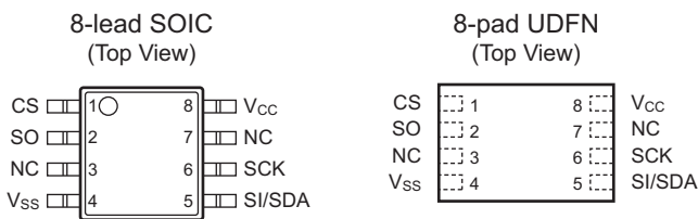
Figure 8-1. Pin Configurations
