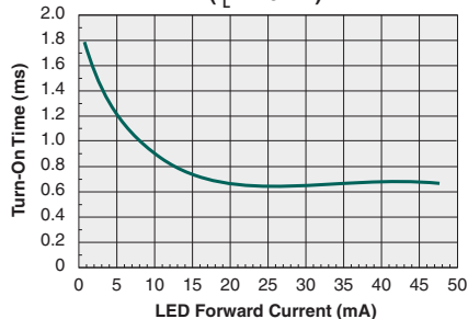
Typical Turn-On Time vs. LED Forward Current ( I_L=120\text{mA} )
