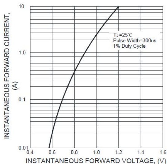
F1G.3-TYPICAL INSTANTANEOUS FORWARD CHARACTERISTICS
