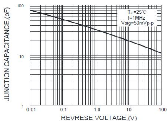
F1G.5-TYPICAL JUNCTION CAPACITANCE
