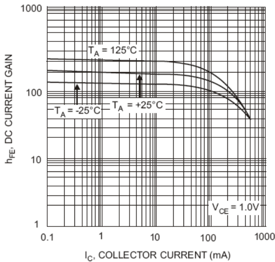
Fig. 3 Typical DC Current Gain vs Collector Current (4401)
