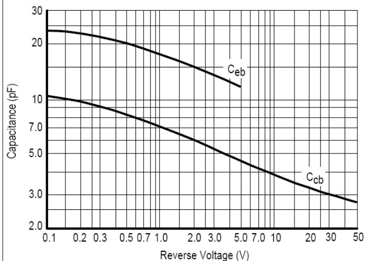
Fig.7 Capacitances
