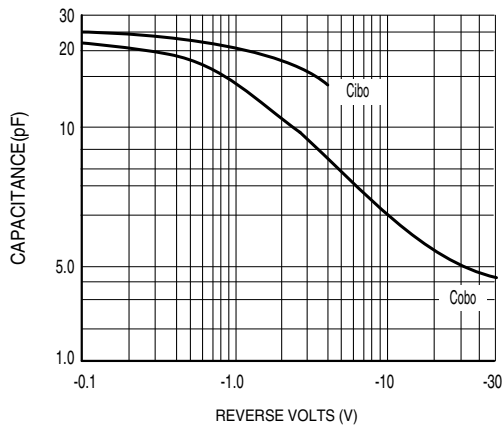
Figure 2.Capacitances(Typical)
