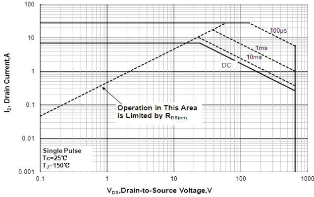
Figure 1 Maximum Forward Bias Safe Operating Area
