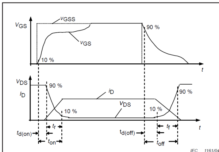
Figure 31. Resistive Switching Time Description
