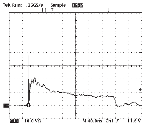
Figure 2. Positive 8 kV contact per IEC 6100 -4-2 - ESD5Z5.0
