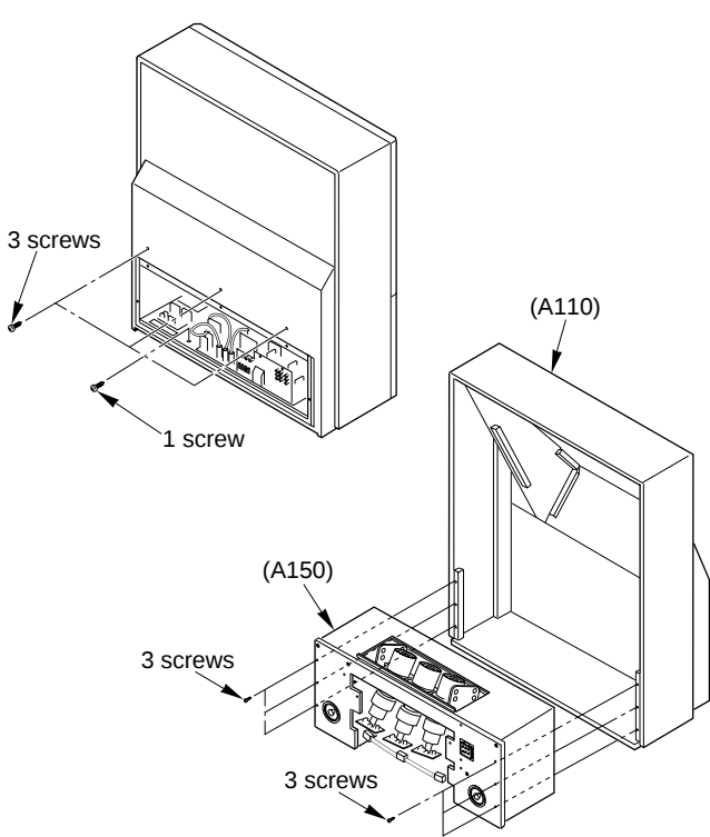
8 Light Box Removal
