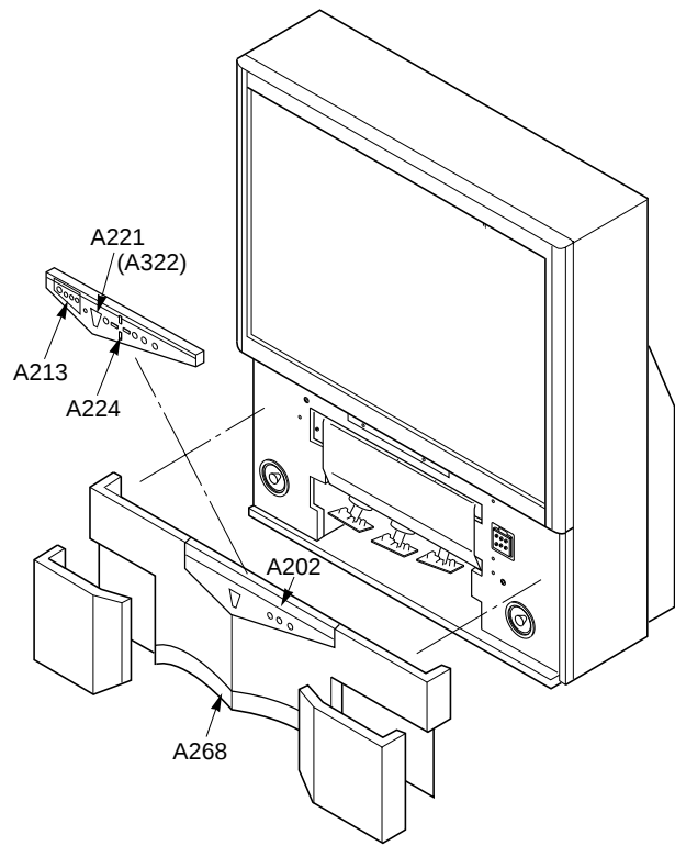
6 Mirror Removal
