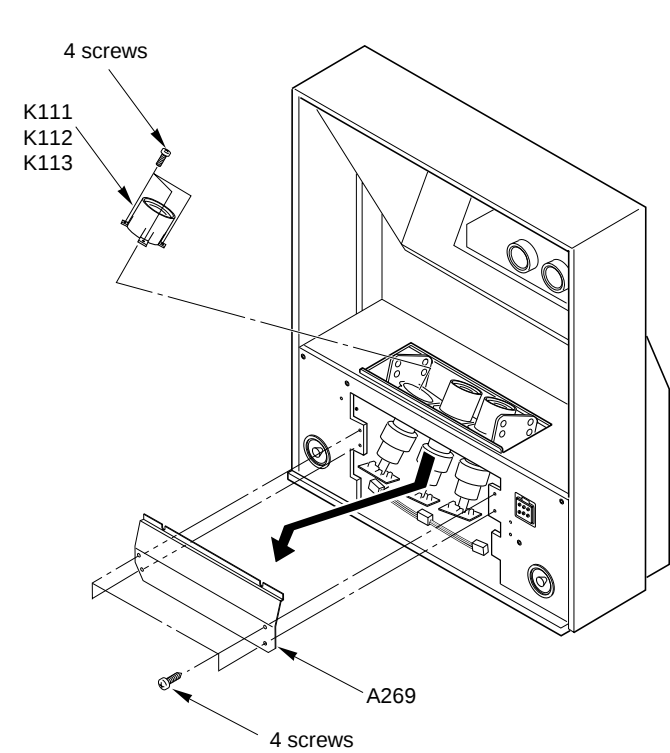
5 Shield Plate, Lens Removal
