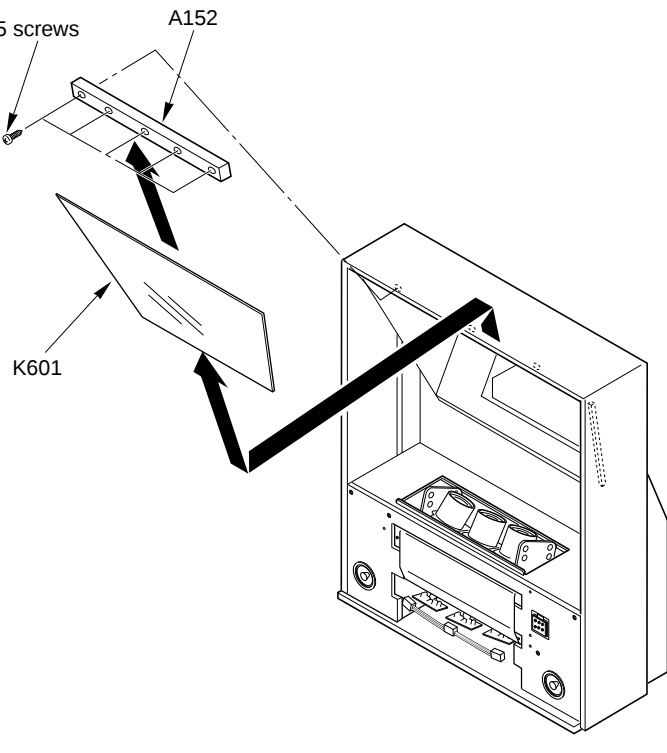
6 Mirror Removal
