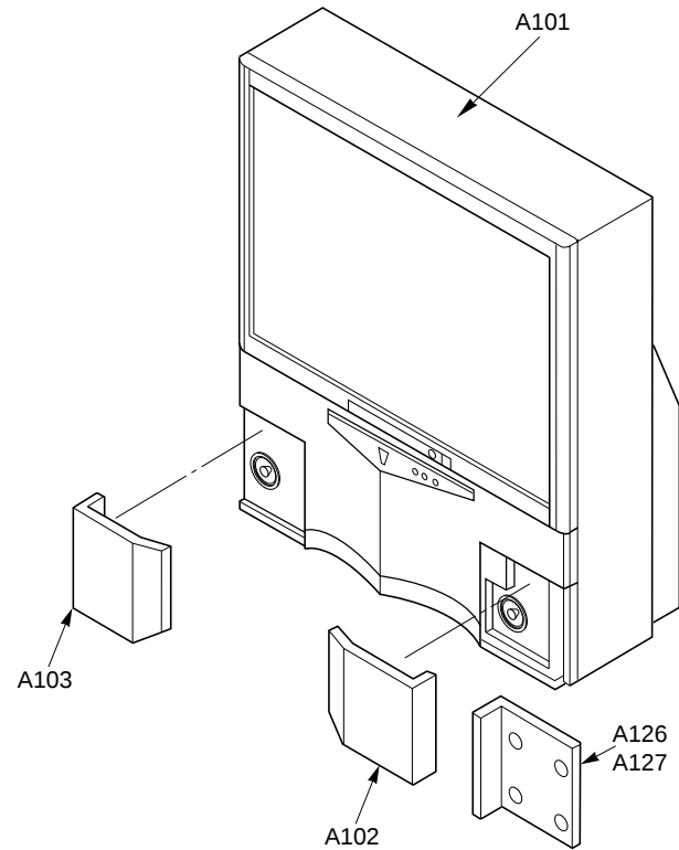
5 Shield Plate, Lens Removal
