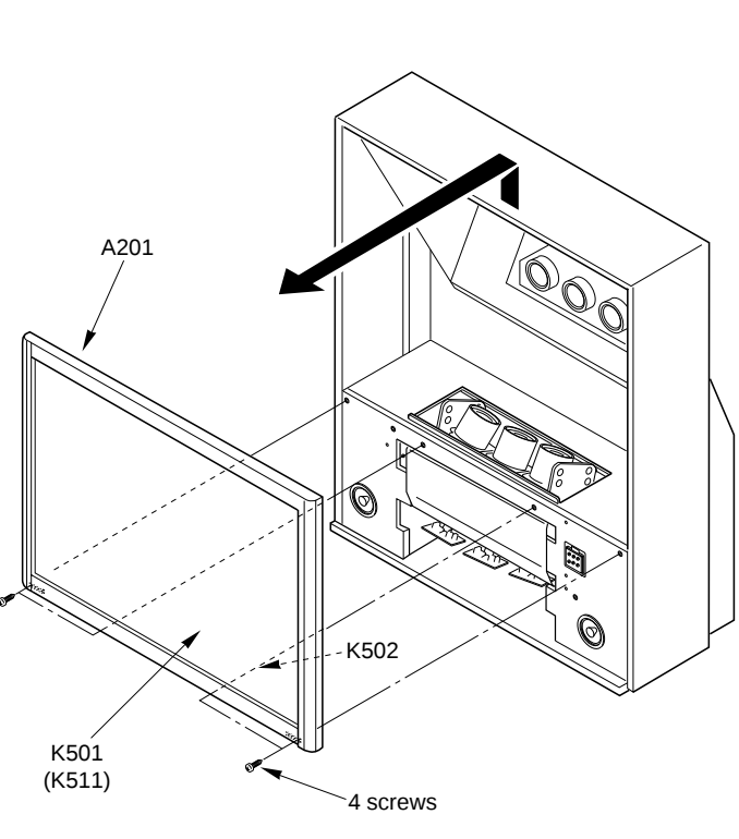
7 Back Board Removal
