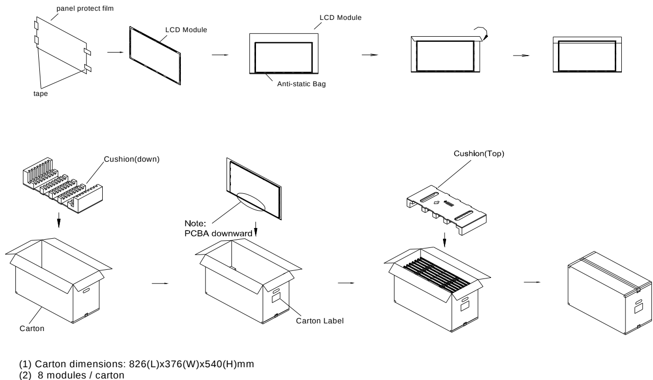
Figure. 8-1 Packing method
