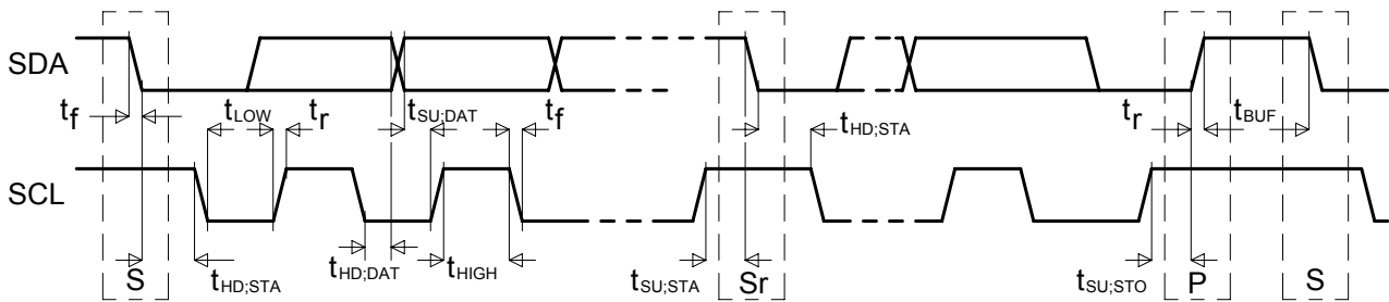
Figure 3-4. Definition of timing for F/S-mode devices on the I 2 C-bus
