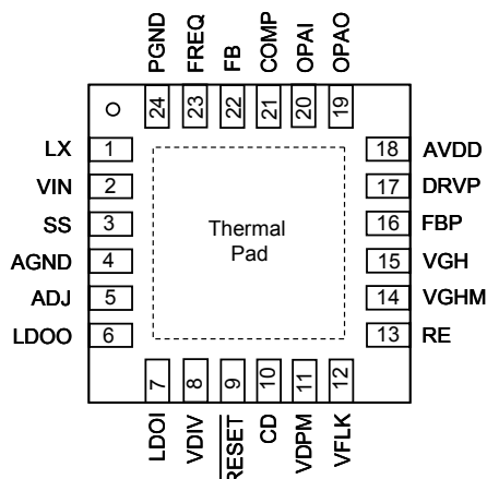
G5521 TQFN4X4-24
