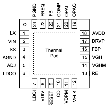
G5521A TQFN4X4-24
