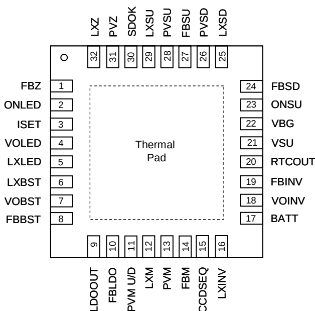
G2202/G2202B TQFN4X4-32
