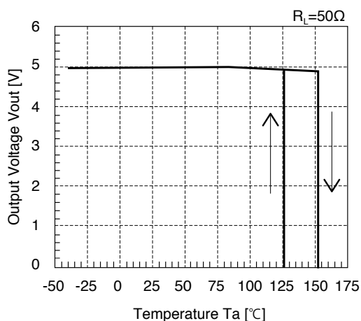
■ OutputVoltage Temperature Coefficient
