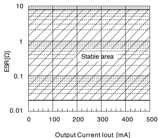
■ ESR stability area
