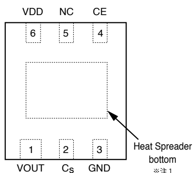
SSON-6A TOP VIEW
