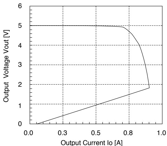
■ Output Current -Output Voltage
