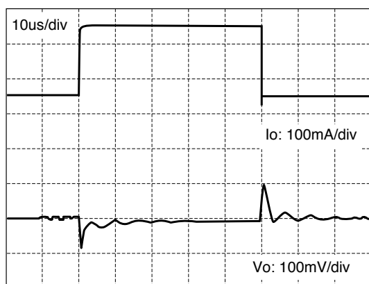
■ Load transient response ( C_{in}=C_o=1\mu F ) I_o: 50mA \leftrightarrow 250mA
