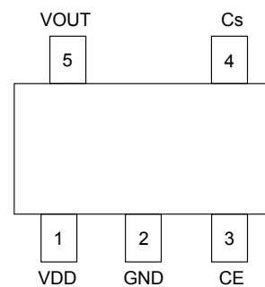
SOT-25A TOP VIEW
