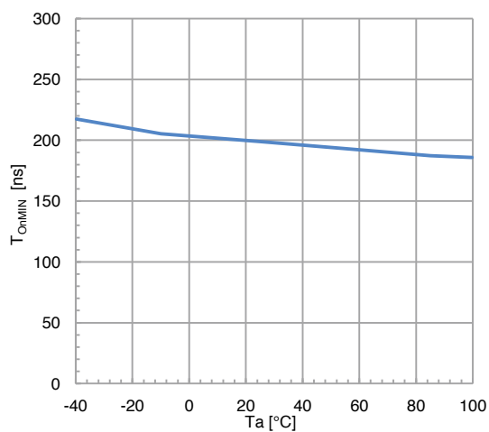
■ Minimum On time vs Temperature
