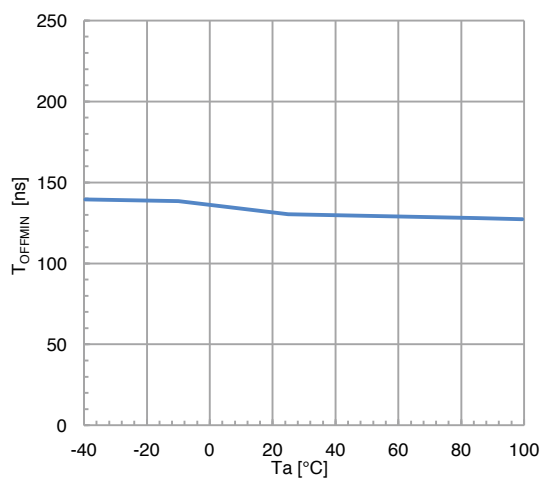
■ Minimum Off time vs Temperature
