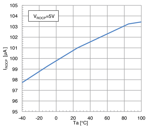
■ ROCP Pin Input Current vs Temperature
