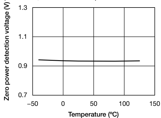
■ Zero power detection voltage - Temperature (VCC=15V, COMP=2V→0V)
