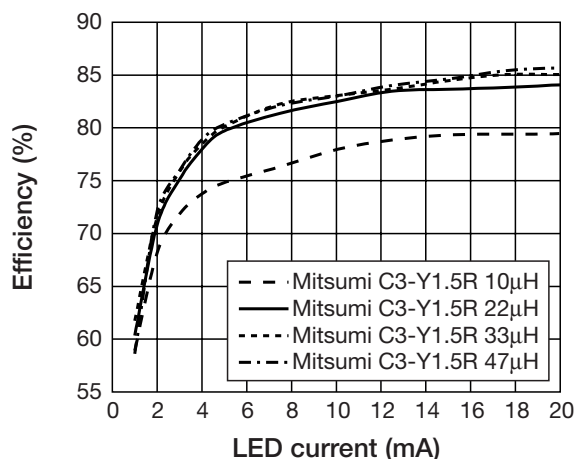
Figure.1 Efficiency comparison of different inductors
