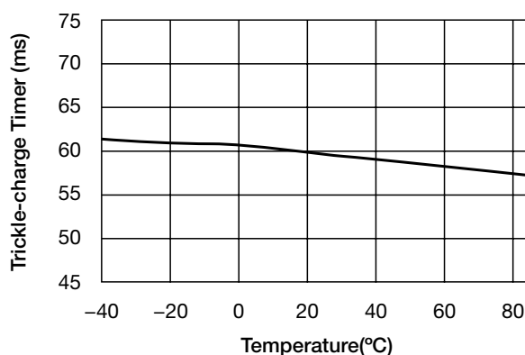
■ Trickle-charge Timer
