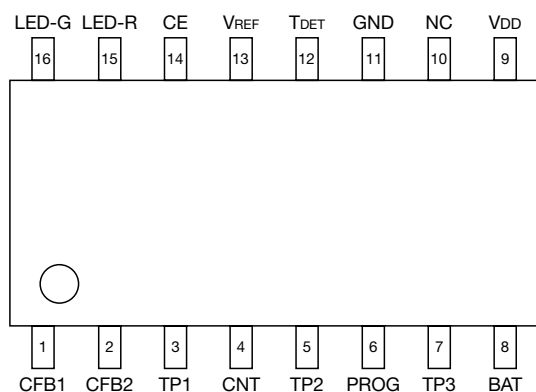
TSOP-16D (TOP VIEW)
