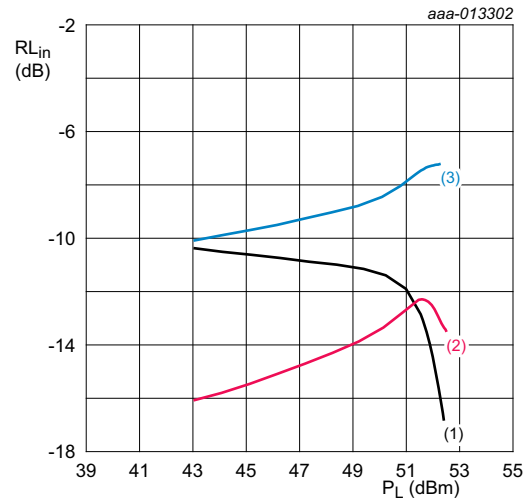
V_{DS} = 28\text{ V}; I_{Dq} = 800\text{ mA}. (1) f = 1805\text{ MHz} (2) f = 1842.5\text{ MHz} (3) f = 1880\text{ MHz}
