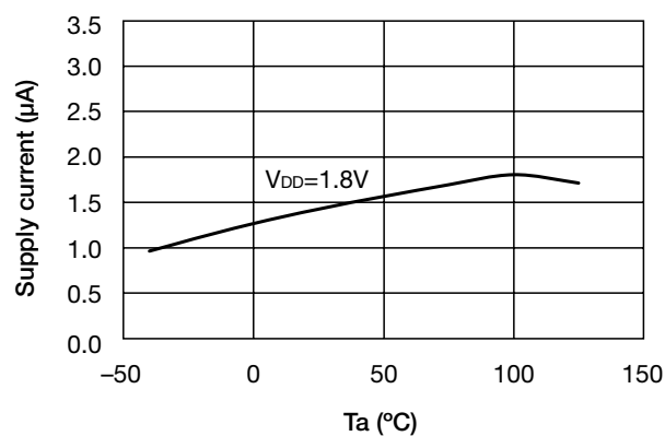
■ Ambient Temparture - Supply Current
