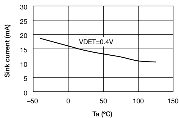
■ Ambient Temparture - DET Sink Current
