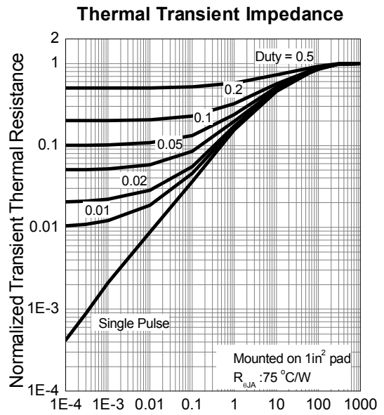
Square Wave Pulse Duration (sec)
