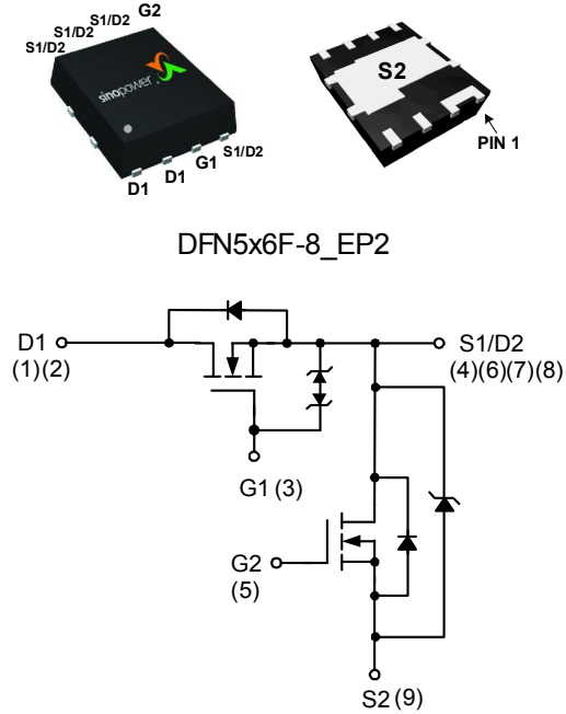
N-Channel MOSFET
