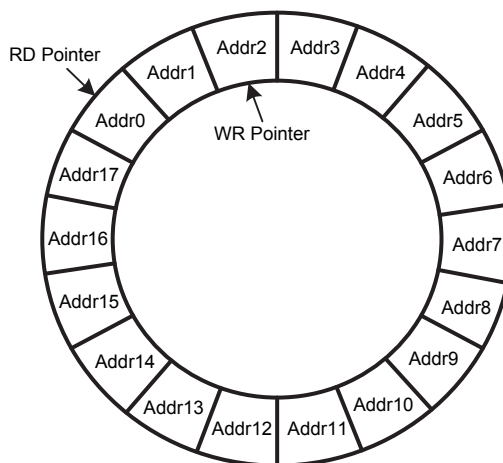
FIFO Structure
