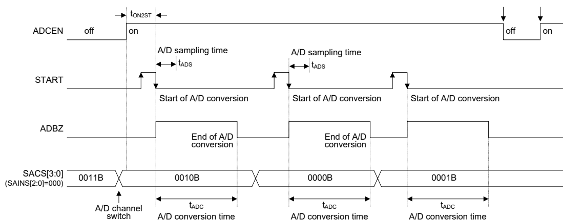
A/D Conversion Timing – External Channel Input
