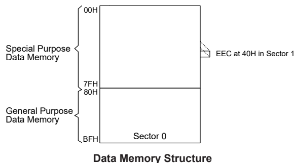
Data Memory Structure
