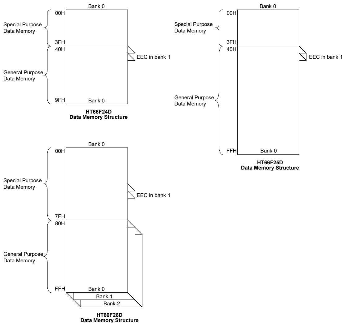
RAM Data Memory Structure
