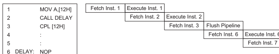
Instruction Fetching
