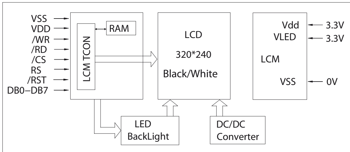
Figure 1. Block diagram
