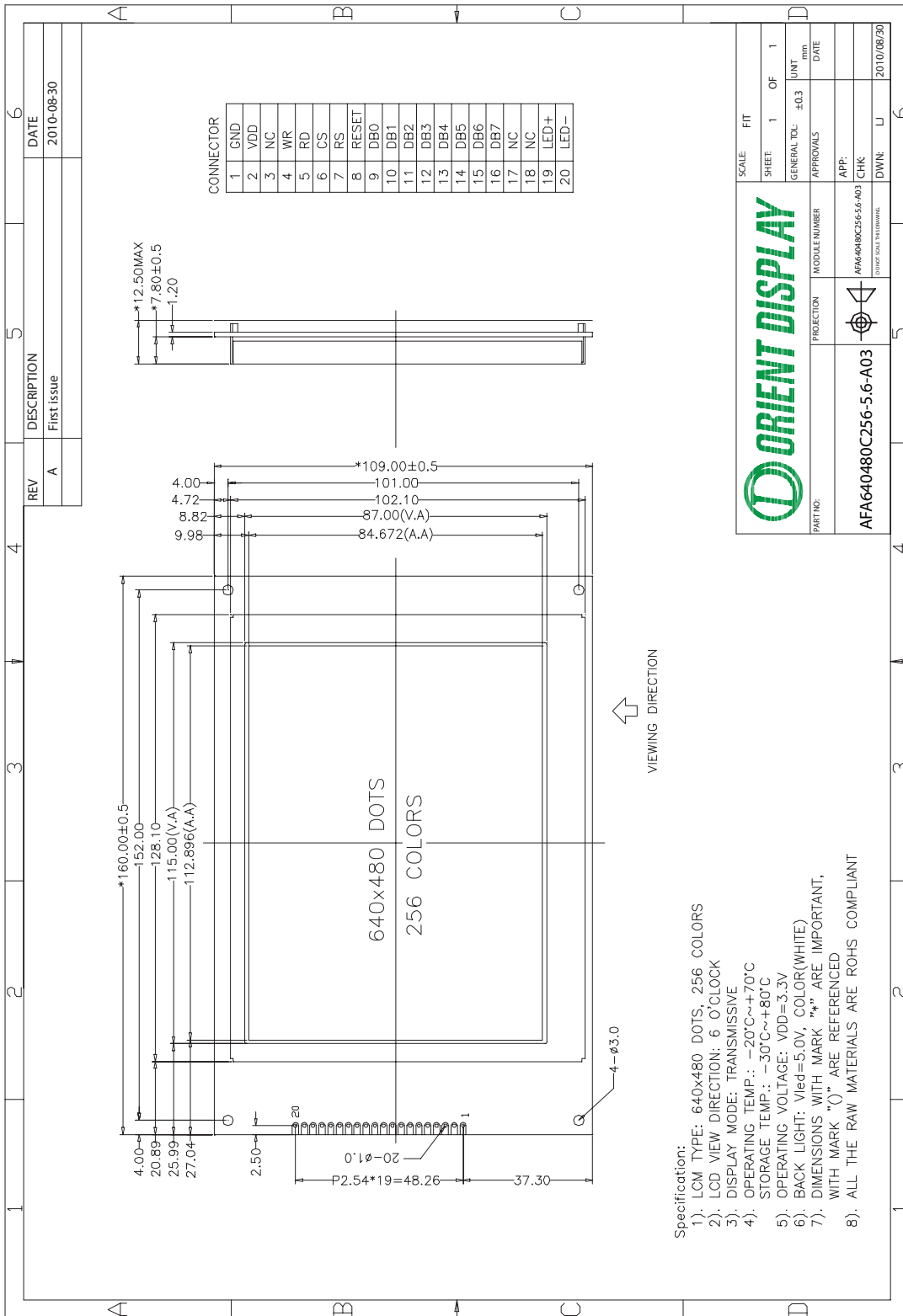
Figure 2. Dimensional outline
