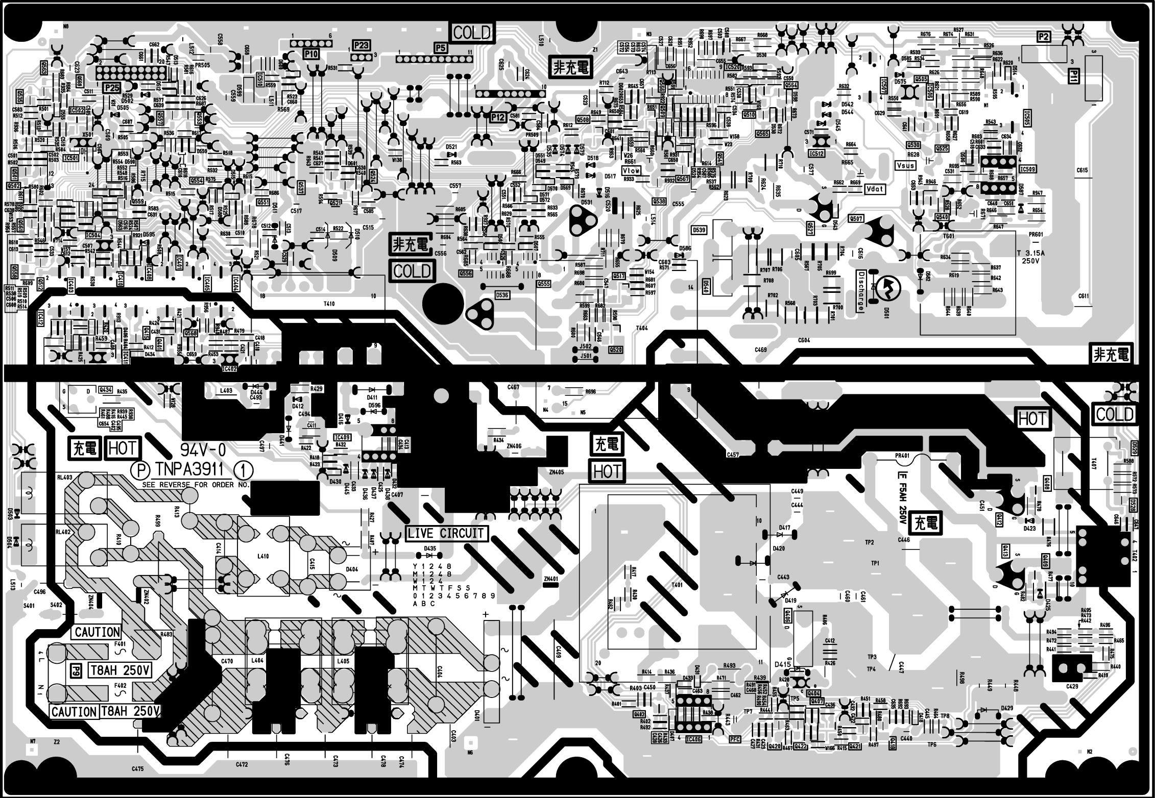
P-BOARD (FOIL SIDE) TNPA3911AL
