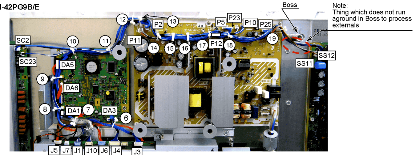
Clamp position
