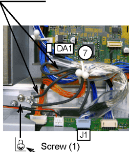
Earth lead
