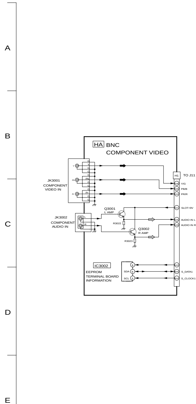
TH-37/42PG9W HA-Board Block and Schematic Diagram
