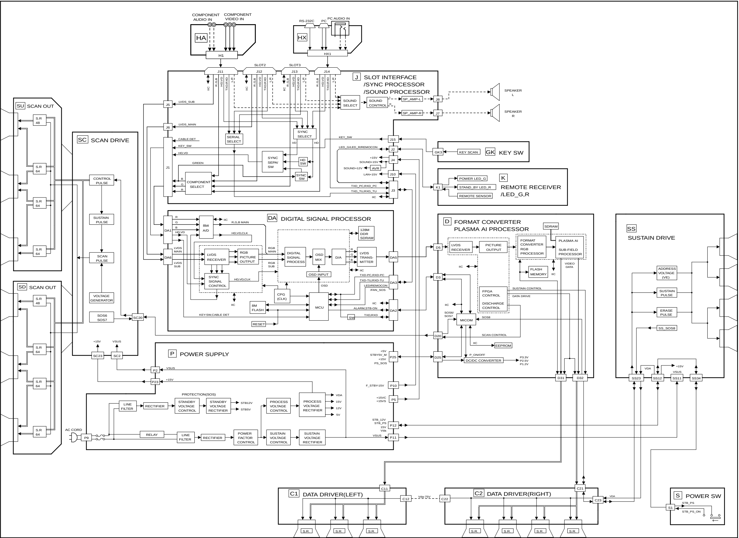
TH-37/42PG9W Main Block Diagram
