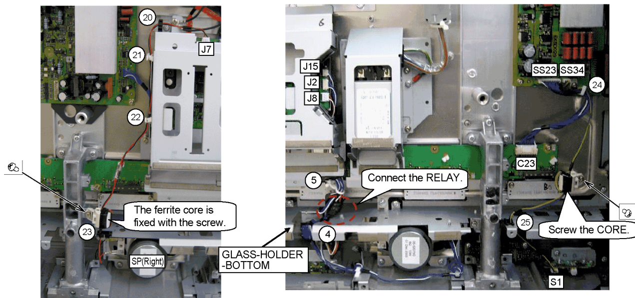
Clamp position
