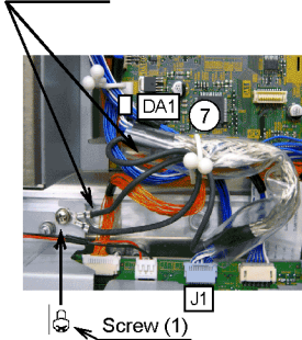
Earth lead
