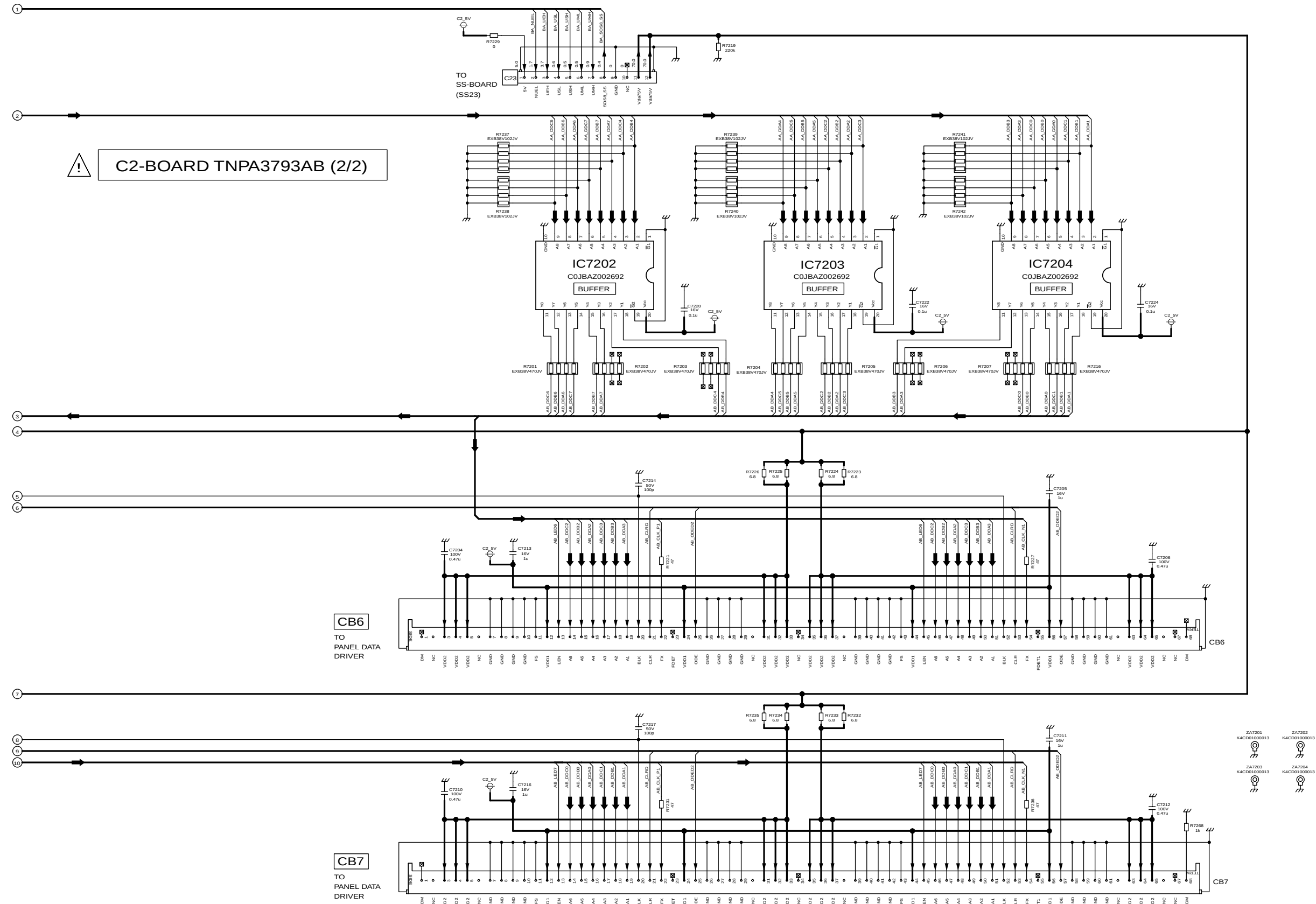
TH-37PG9W C2-Board (2 of 2) Schematic Diagram
