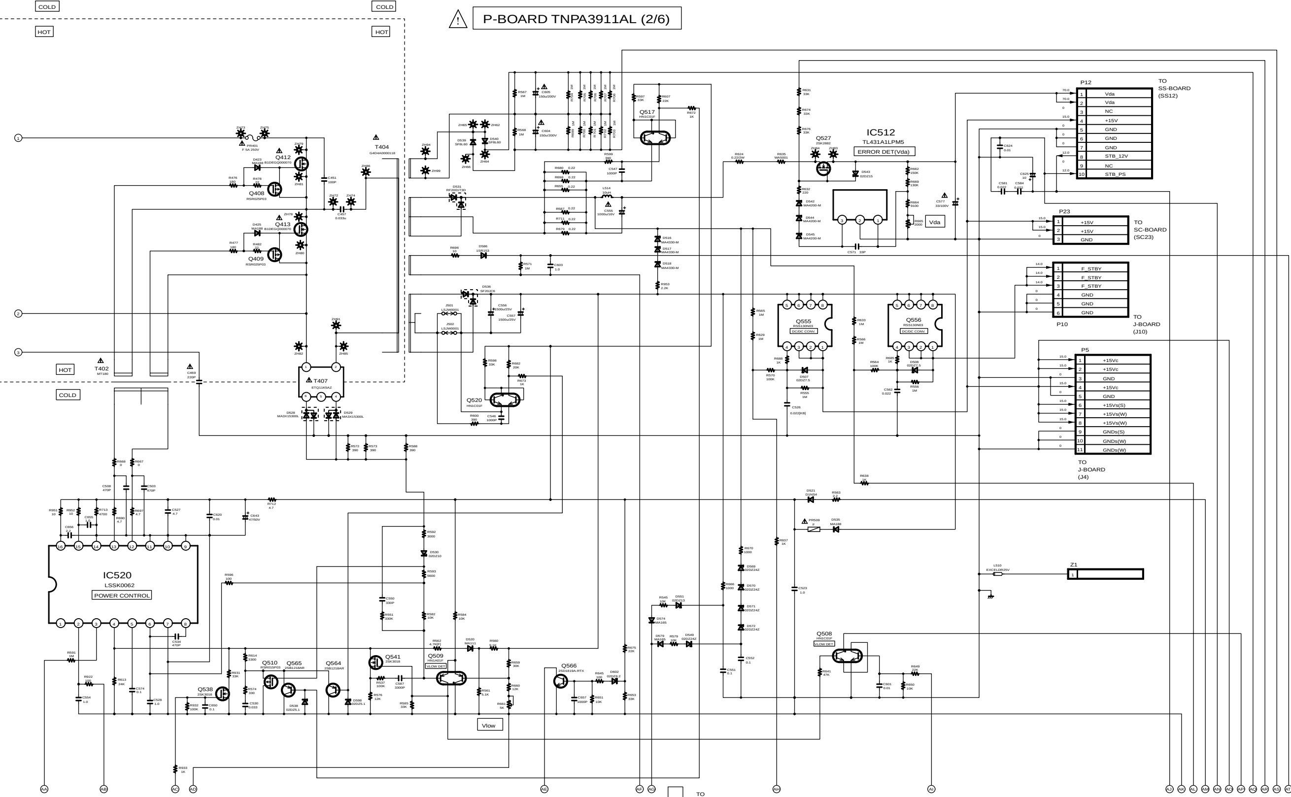
TH-42PG9W P-Board (2 of 6) Schematic Diagram
