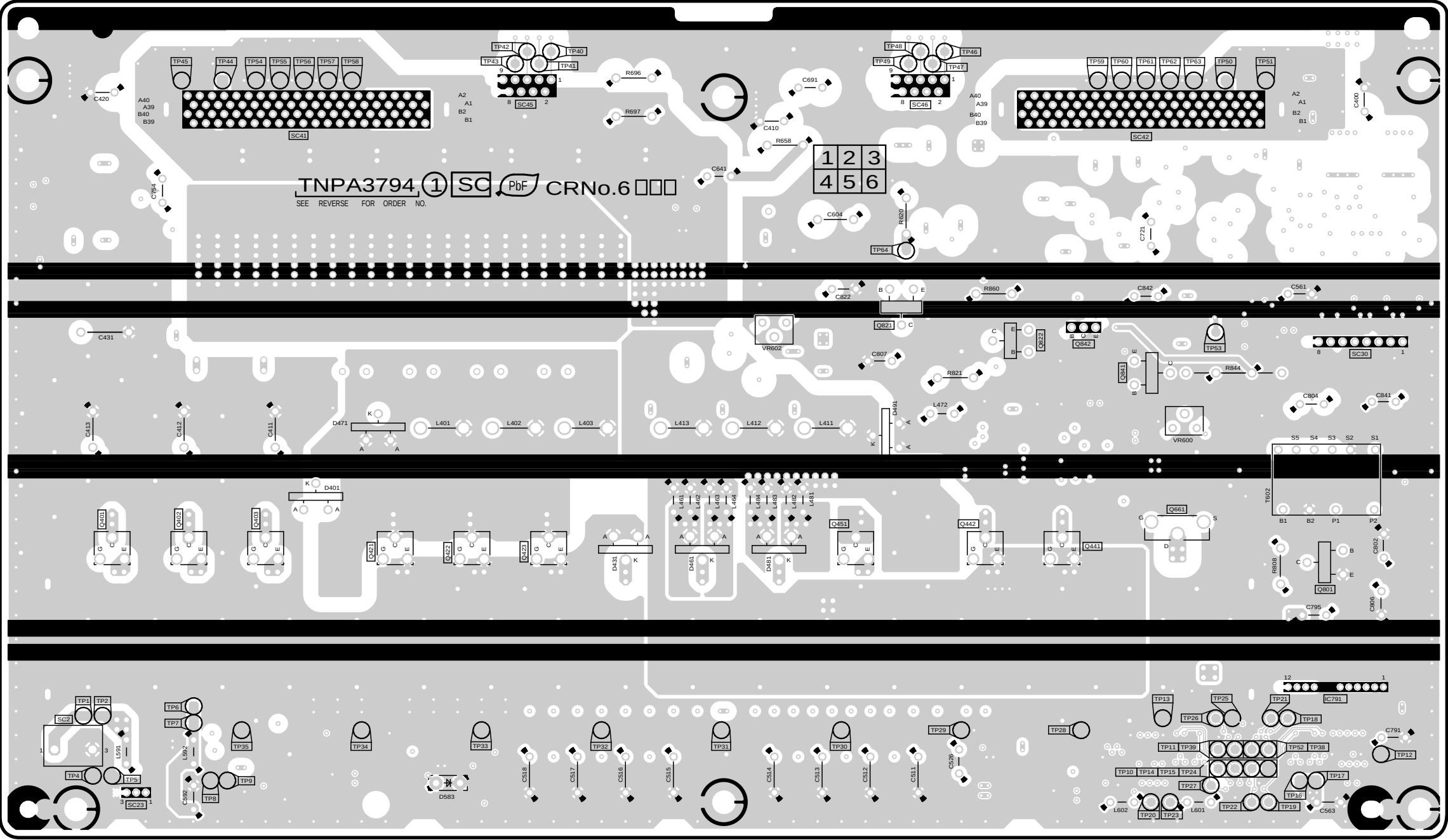
SC-BOARD (FOIL SIDE) TNPA3794AE (37inch) TNPA3794AB (42inch)
