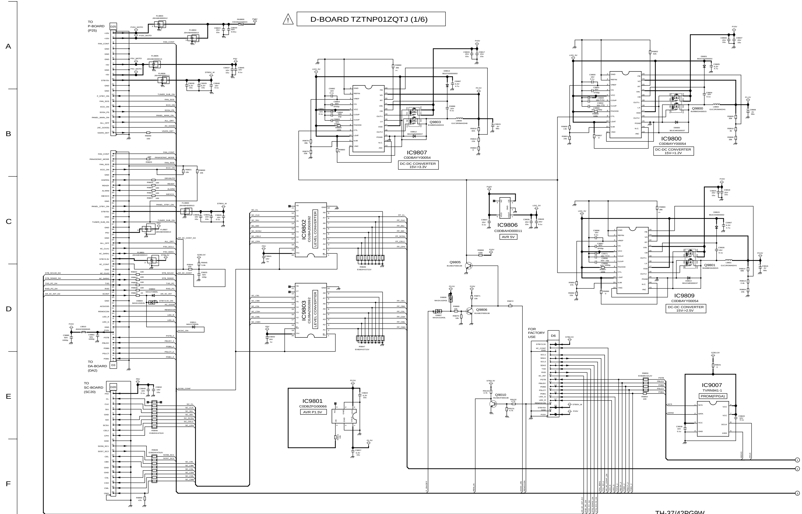
TH-37/42PG9W D-Board (1 of 6) Schematic Diagram
