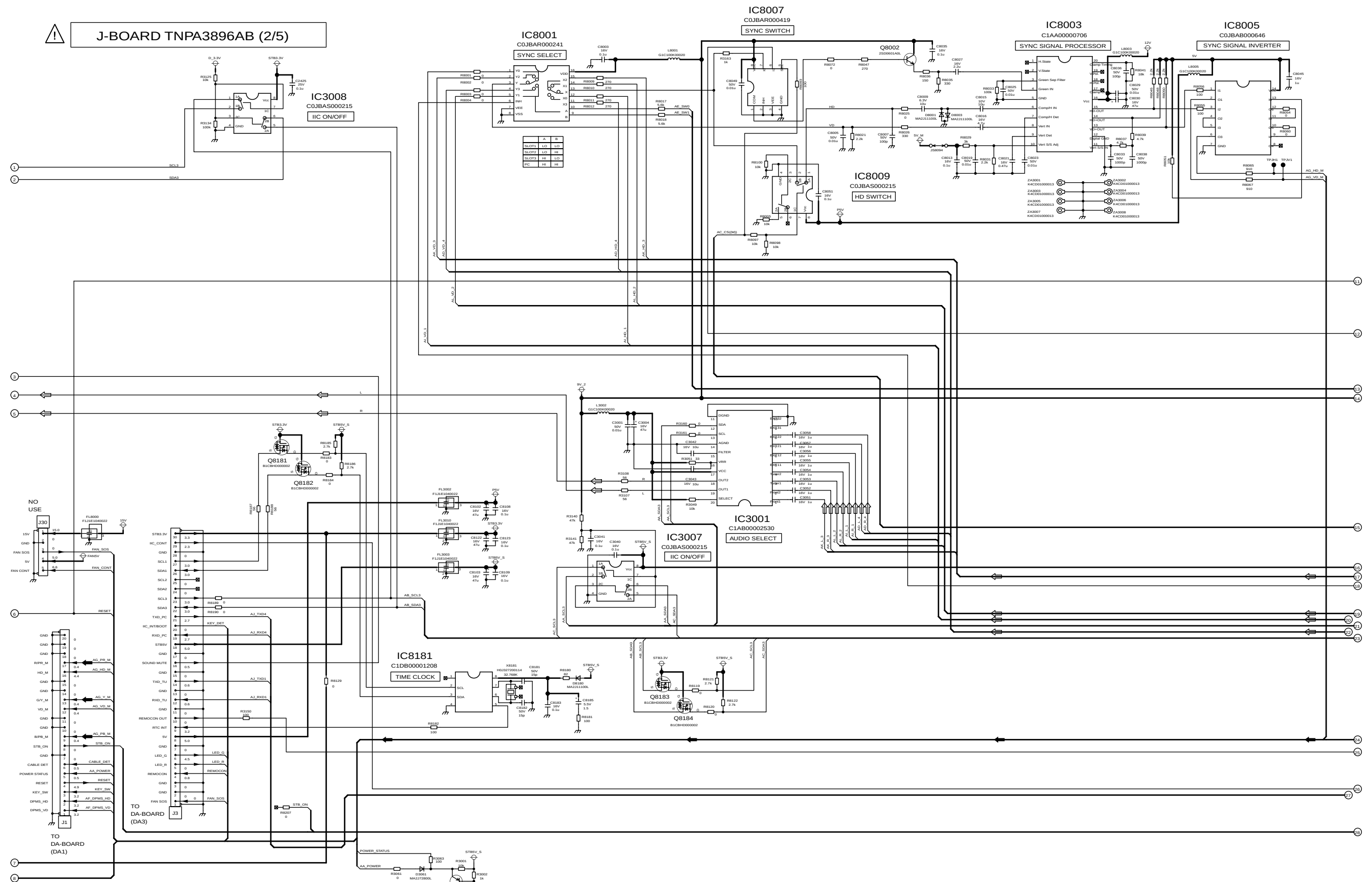
TH-37/42PG9W J-Board (2 of 5) Schematic Diagram
