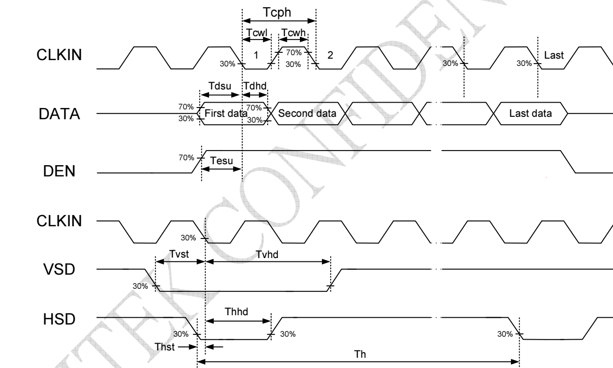
Source output timing diagram
