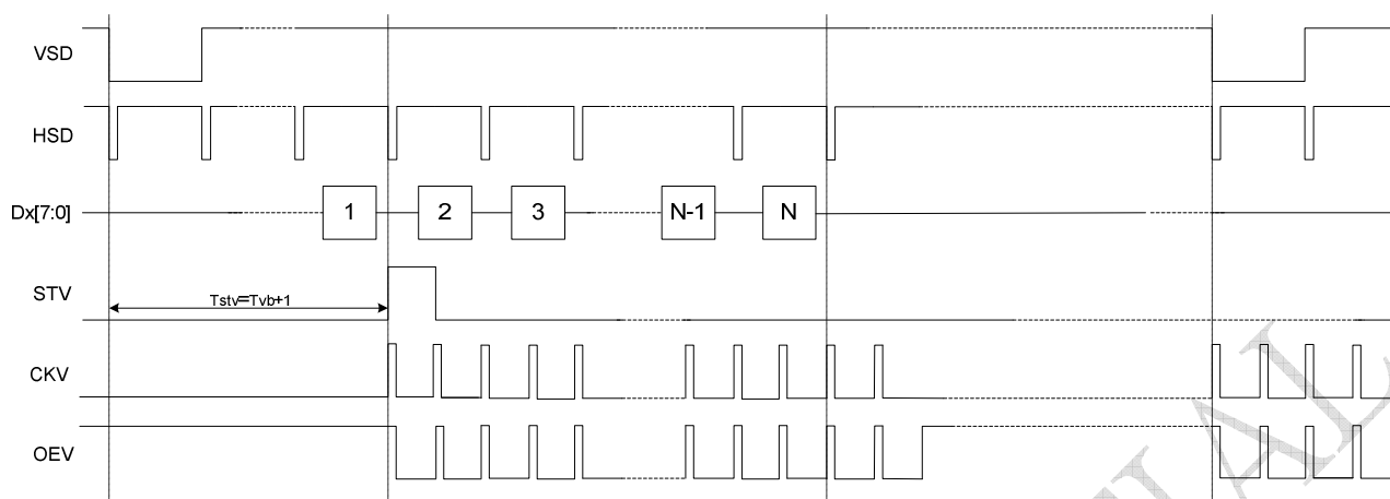
Vertical Timing Diagram of HV Mode (Dual Gate)
