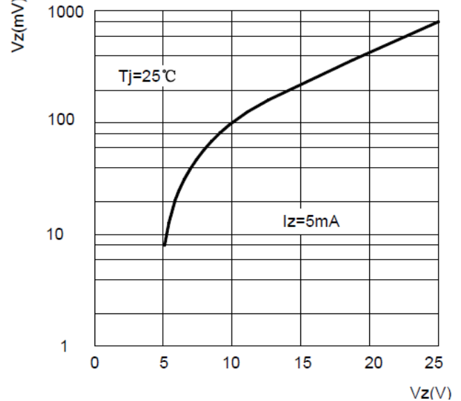
FIG2: Typical Change of Working Voltage under Operating Conditions at T_{amb}=25^{\circ}C
