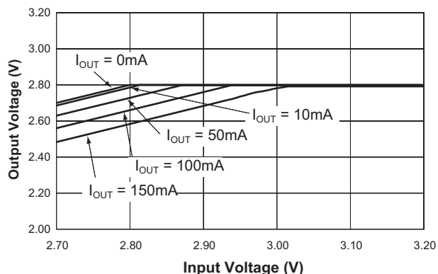
Dropout Characteristics
