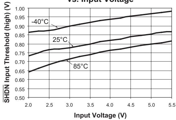
\overline{SHDN} Input Threshold (high) vs. Input Voltage
