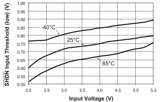
\overline{SHDN} Input Threshold (low) vs. Input Voltage
