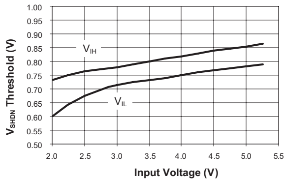
V_{SHDN} Threshold vs. Input Voltage
