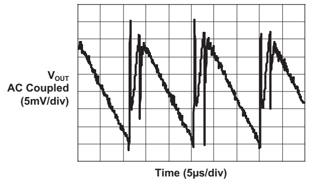
Output Ripple ( I_{OUT} = 100mA @ V_{IN} = 3.0V )
