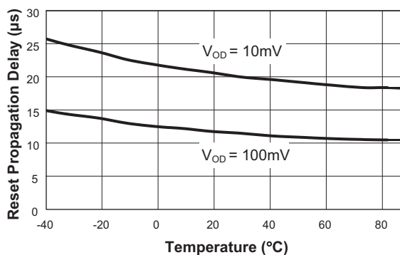
Power-Down Reset Propagation Delay vs. Temperature
