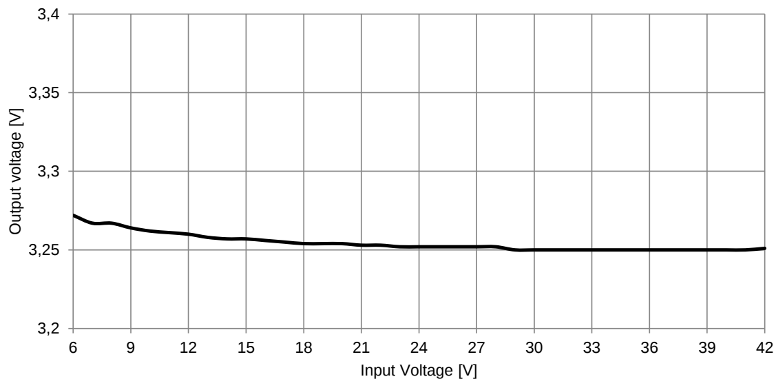
171020601 Line Regulation V_{OUT} = 3.3V , I_{OUT} = 2A , T_A = 25^\circ C
