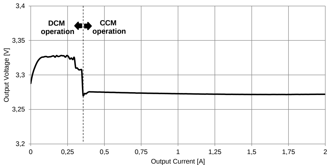
171020601 Load Regulation V_{IN} = 24V , V_{OUT} = 3.3V , T_A = 25^\circ C
