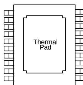
TSSOP-20P (Bottom View)
